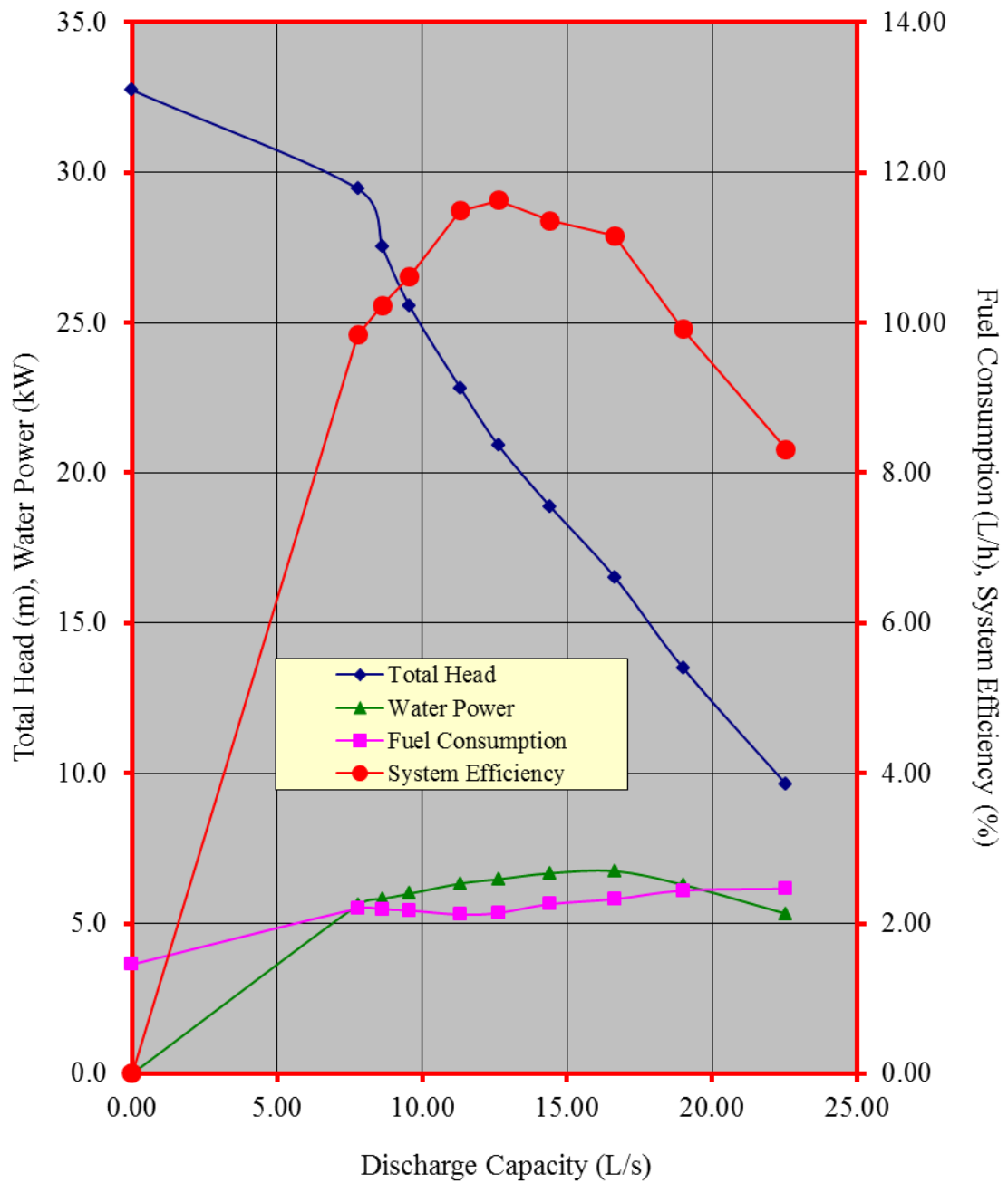
Figure 3. Performance characteristic curves of the KITACO 4 x 4MS centrifugal pump coupled to YANMAR TF90MLY Diesel Engine
